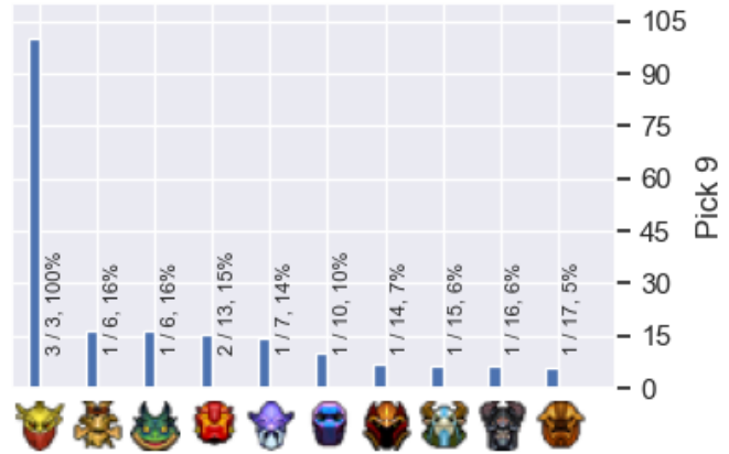
Second pick
