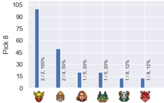
First pick
