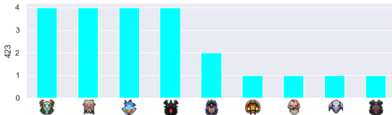
Matches
